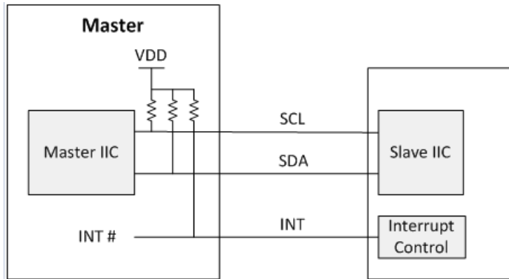
• Figure6. IIC connect for master and HY0110
