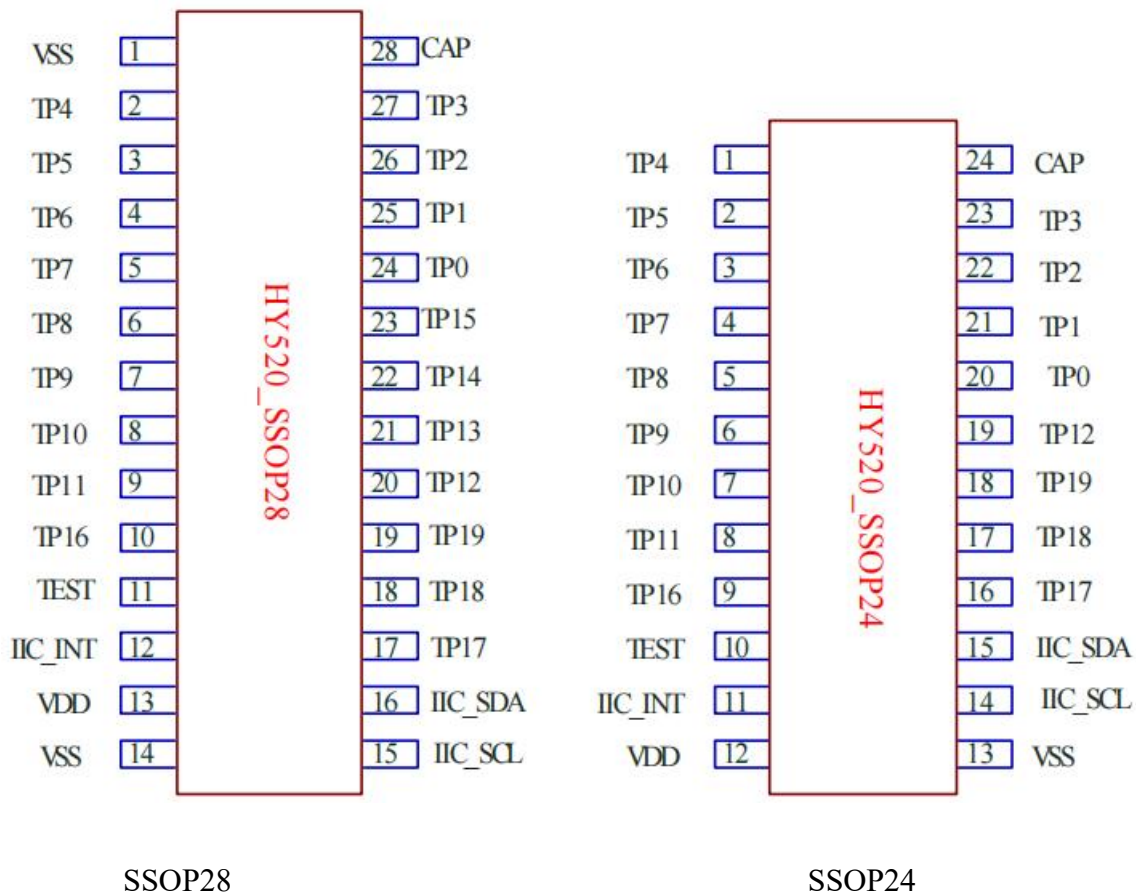
Figure5. pin define for IC package
