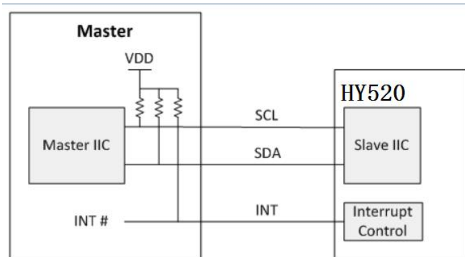
Figure6. IIC connect for master and HY520
