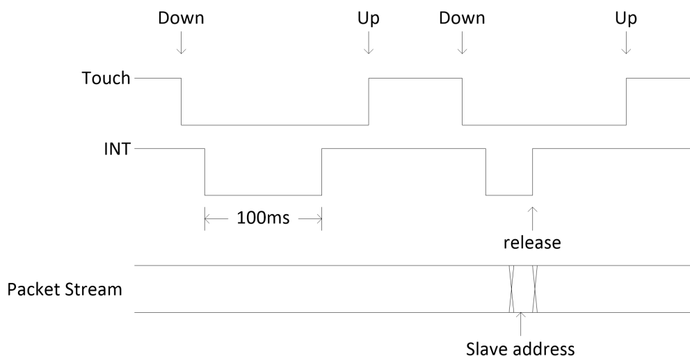
Figure7. INT pin describe
